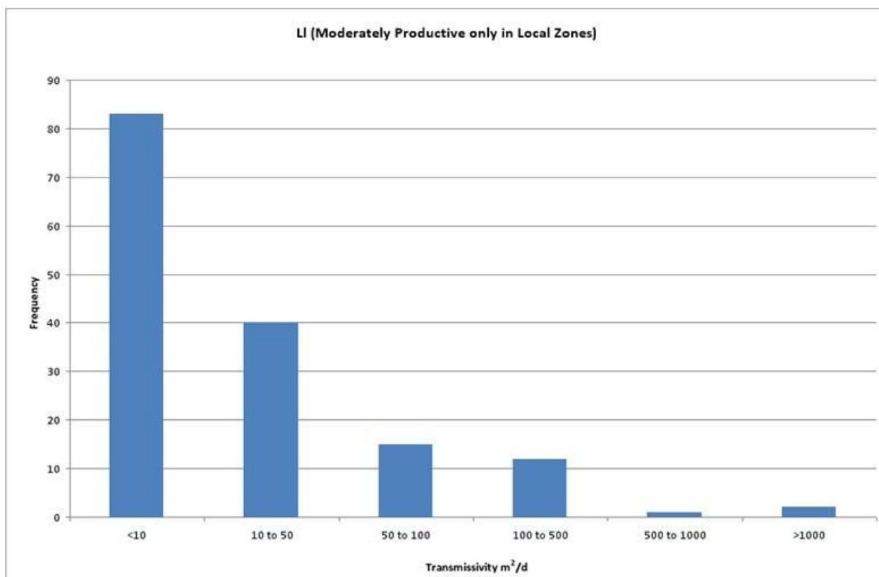
Figure 4. Preliminary frequency plot of transmissivity for Locally Important Bedrock Aquifers which are Moderately Productive only in Local Zones (LI)
