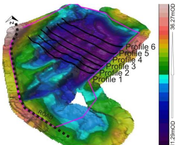
Figure 8. Topography contours. Vertical exaggeration x 3.
