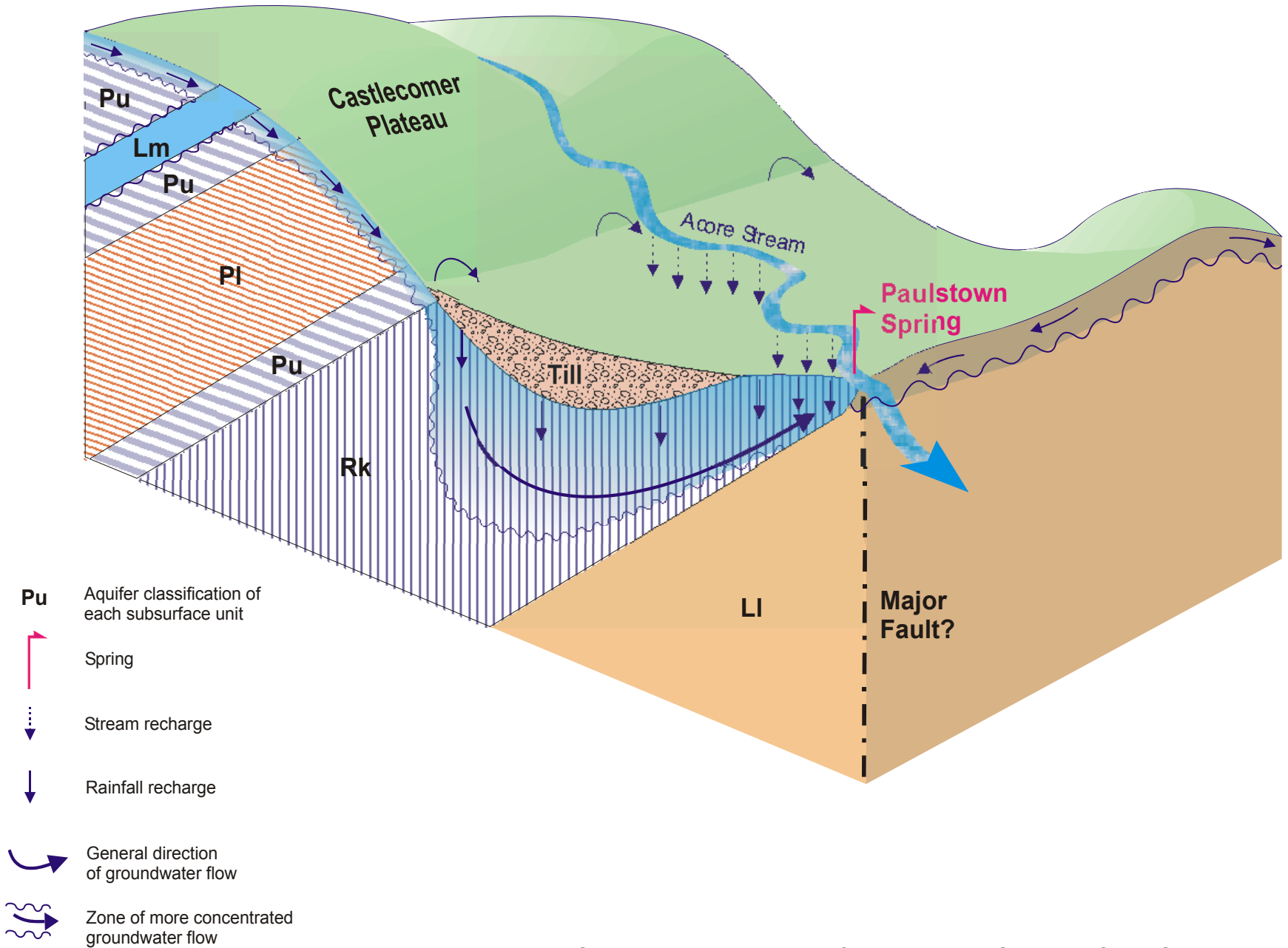
Figure 11.1 Schematic Hydrogeology of the Paulstown Source in Cross Section
