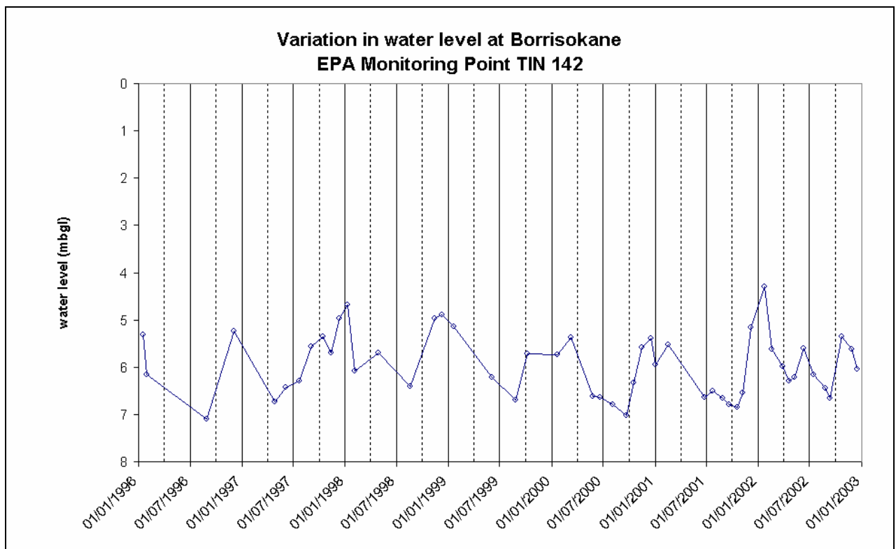
Figure 1: Groundwater hydrograph
