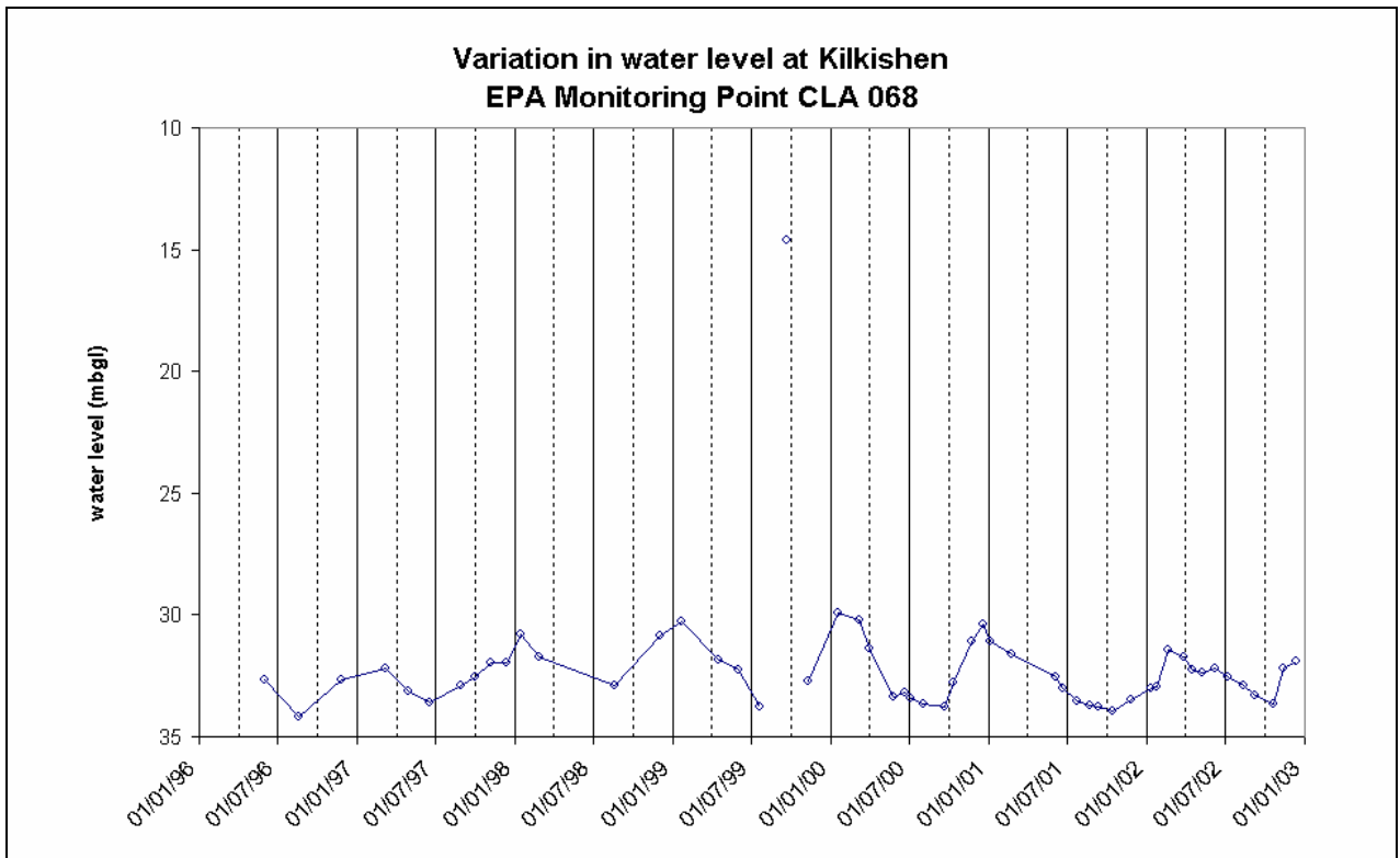
Figure 1: Groundwater hydrograph
