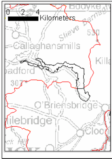
Figure 1. Location and boundaries of Glenomra Gravels. Red line is hydrometric boundary.
