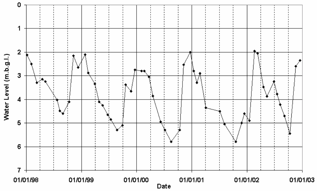
Well Hydrograph at EPA Monitoring Station Coolrain (LAC069)
