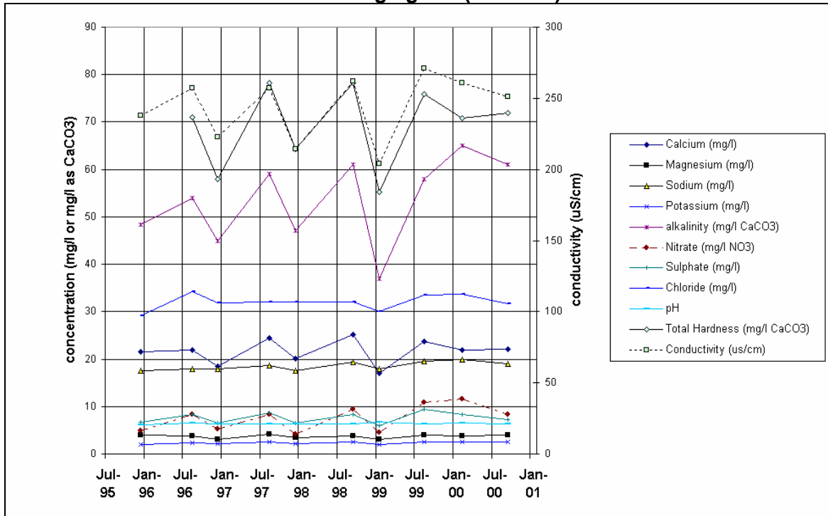
Figure 2: Seasonal variation of major hydrochemical parameters at Ballinloghig WS (KER 005)
