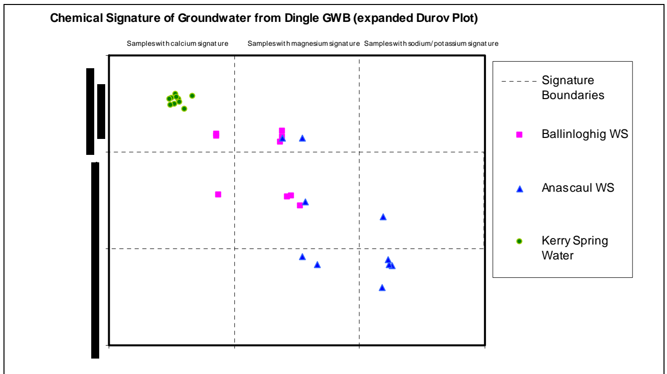
Figure 1: Hydrochemical signature (EPA Representative Monitoring)
