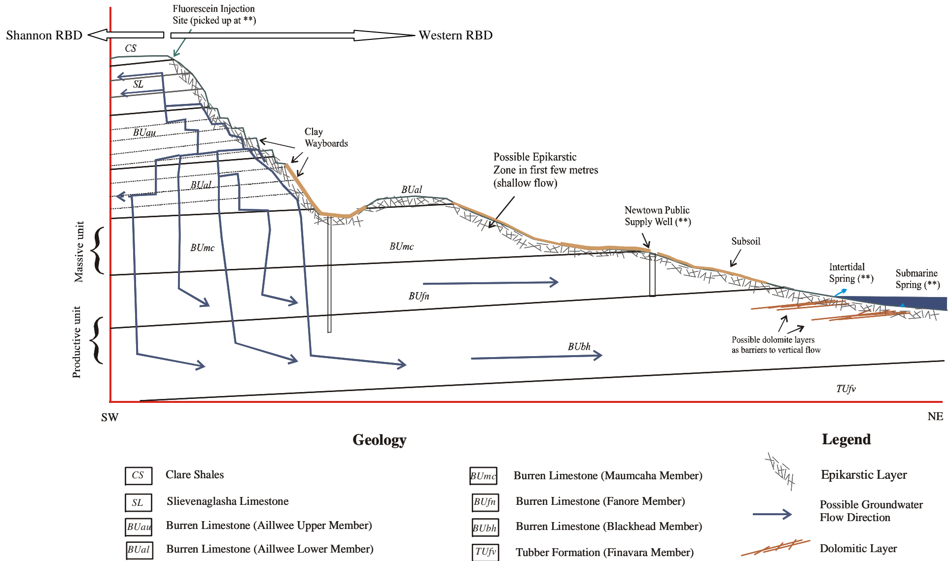
Figure 2: Schematic diagram of groundwater flow from Burren uplands (i) north to the Ballyvagh area (Western RBD) and (ii) south to the Elmvale springs (Shannon RBD)
